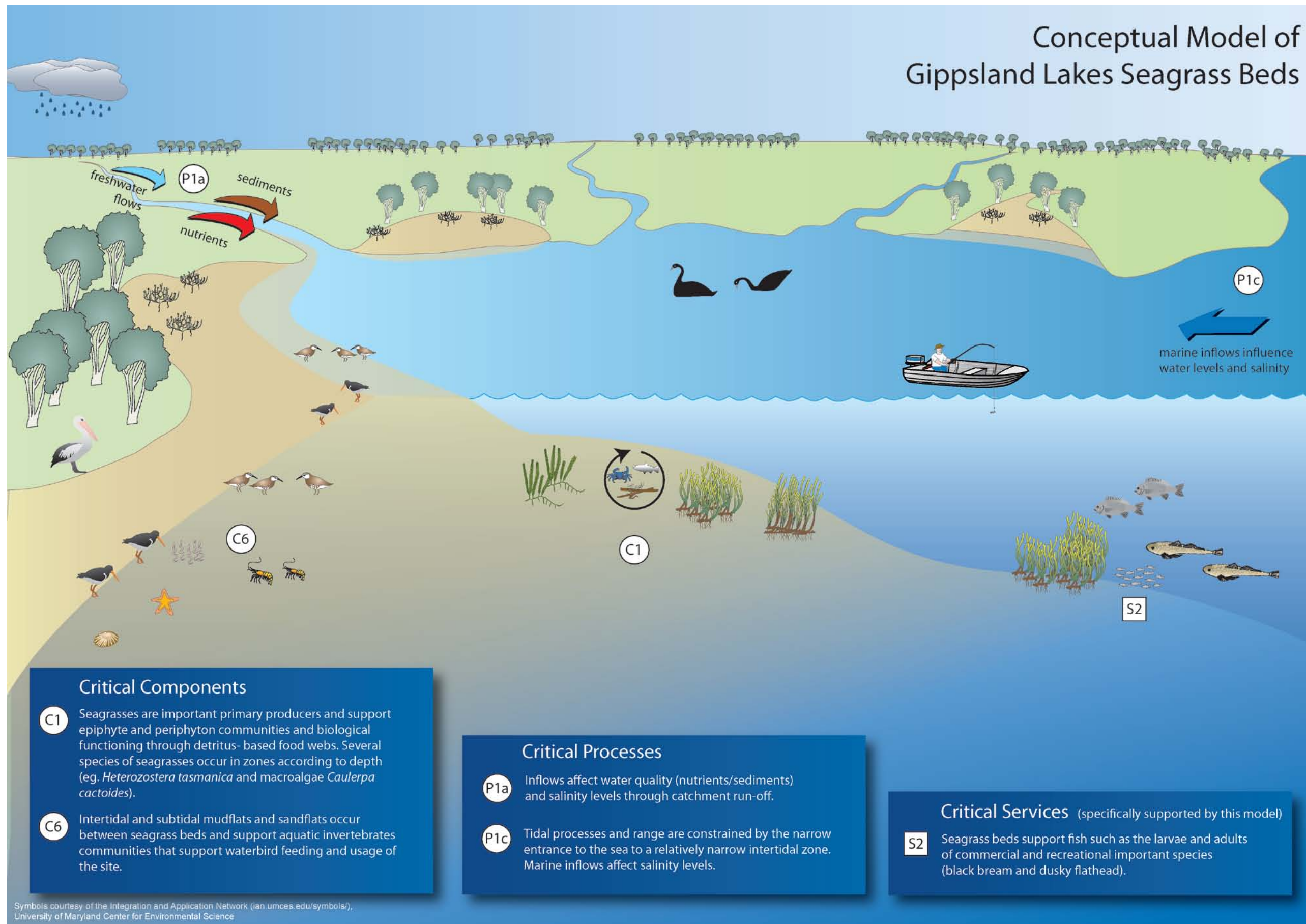
Figure 3-1 Conceptual model of Gippsland Lakes seagrass beds
